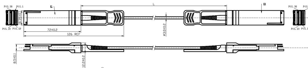
Figure 4, Mechanical Diagram
