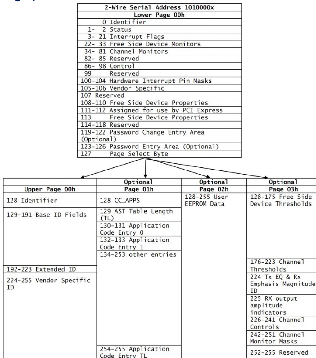
Figure 3, Memory Map
