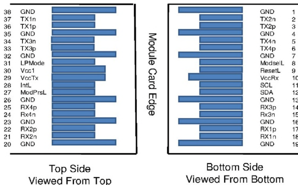
Figure 2, Pin View
