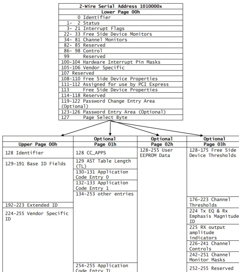
Figure 3, Memory Map
