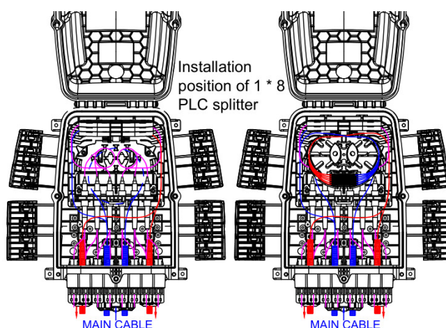
Pic 3 Cable ways
