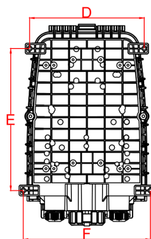
Pic 2 Installation Size
